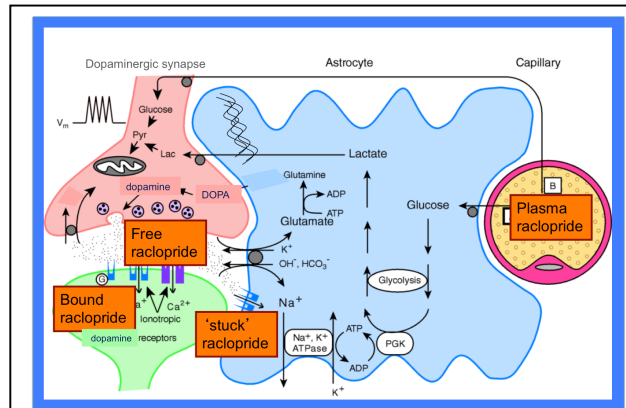
Figure 3. Possible states of an injected radiotracer. The states can be thought of as distinct, interconnected pools. Figure modified (Pellerin & Magistretti, 1994).
