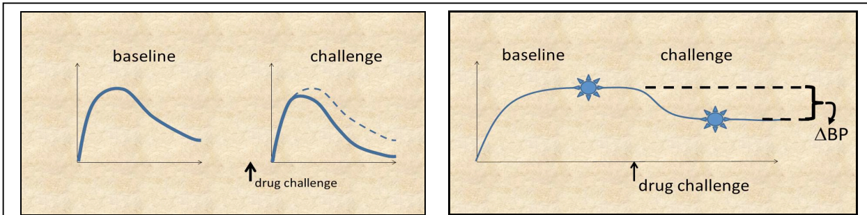
Figure 10. Two common schemes for measuring change in BP with PET. General appearance of data from a paired bolus study (left) compared to a single bolus plus infusion study (right). Stars on right indicate that only two static measurements are necessary to get change in BP from an equilibrium study.
