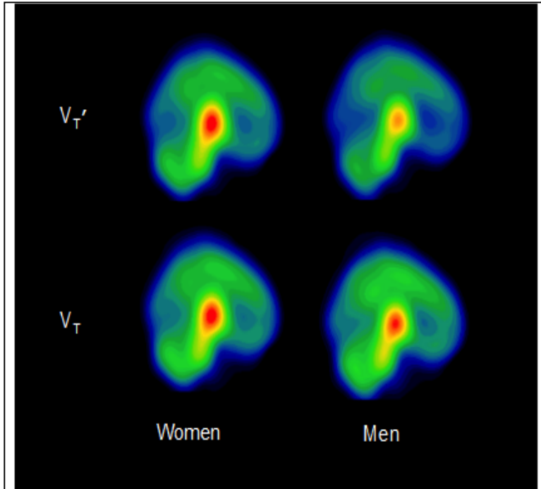
Figure 16. Mean parametric images illustrating ^{123}\text{I} -5-IA-85380 activity in 10 men and 19 women in V_T' (regional activity divided by total plasma parent between 6 and 8 h) and V_T (regional activity divided by free plasma parent between 6 and 8 h). Across brain regions, the main V_T' component was significantly greater in women than in men, but the main V_T component did not significantly differ between the sexes. This research was originally published in JNM . 123I-5-IA-85380 SPECT Imaging of Nicotinic Acetylcholine Receptor Availability in Nonsmokers: Effects of Sex and Menstrual Phase. JNM . 2007;48:1637. © by the Society of Nuclear Medicine and Molecular Imaging, Inc.
